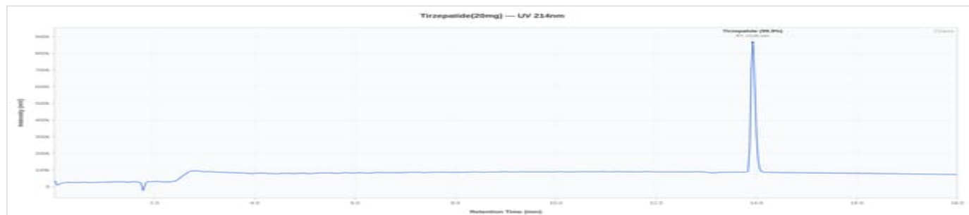
Tirzepatide 20mg - 70126CLTR20: UV Chromatogram
