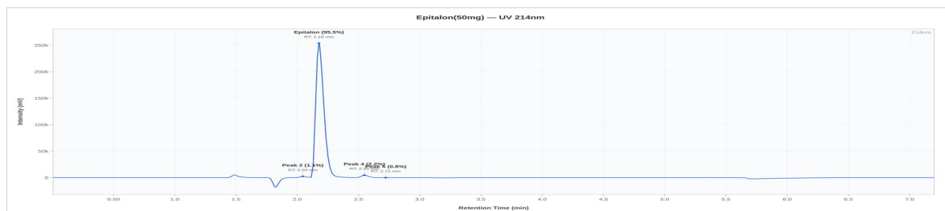
Epitalon 50mg - 70126CLET50: UV Chromatogram
